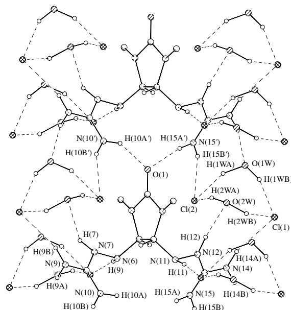
Figure 2 Schematic diagram of a homochiral H-bonded chain along the axis a in the crystal structure of compound 2b . The parameters of H-bonds: OH...Cl [O...Cl 3.056(7)–3.232(7) Å, H...Cl 2.09–2.30 Å, OHCl 134–157°], N–H...O [N...O 2.799(7)–2.937(7) Å, H...O 1.93–2.01 Å, NHO 142–165°], N–H...Cl [N...Cl 3.286(7)–3.418(7) Å, H...Cl 2.42–2.57 Å, NHCl 154–167°].
