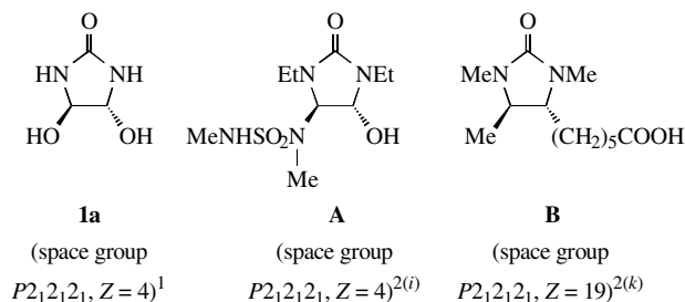
Scheme 1 Conglomerates of imidazolidin-2-ones.
