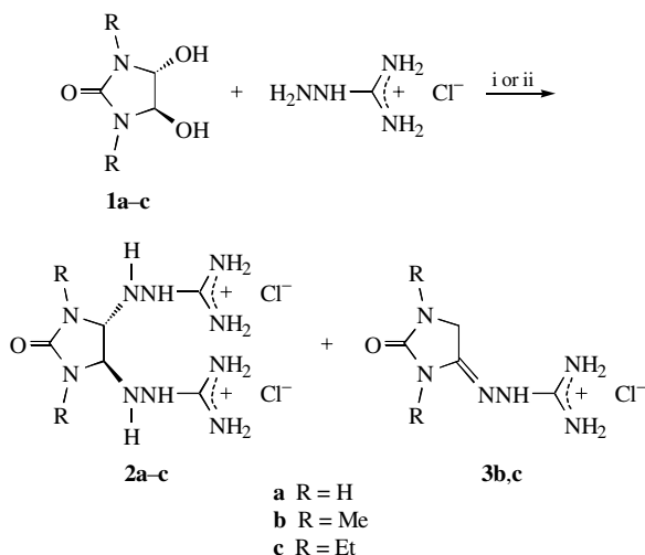
Scheme 2 Reagents and conditions: i, H 2 O, pH 1–2, 80 °C, 1 h; ii, MeOH, conc. HCl, 60 °C, 1 h.
