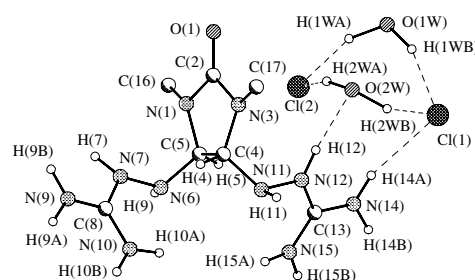
Figure 1 The molecular structure of compound 2b . Main bond lengths (Å): O(1)–C(2) 1.218(5), N(1)–C(2) 1.381(8), N(1)–C(5) 1.463(6), C(2)–N(3) 1.374(8), N(3)–C(4) 1.455(6), C(4)–N(11) 1.452(6), C(4)–C(5) 1.545(5), C(5)–N(6) 1.430(6), N(6)–N(7) 1.402(7), N(7)–C(8) 1.346(6), C(8)–N(9) 1.313(7), C(8)–N(10) 1.323(7), N(11)–N(12) 1.384(6), N(12)–C(13) 1.340(6), C(13)–N(15) 1.320(7), C(13)–N(14) 1.340(7); valence angles (°): C(2)–N(1)–C(5) 110.4(4), C(2)–N(1)–C(16) 121.5(4), C(5)–N(1)–C(16) 121.0(4), O(1)–C(2)–N(3) 126.2(6), O(1)–C(2)–N(1) 125.2(6), N(3)–C(2)–N(1) 108.6(3), C(2)–N(3)–C(4) 110.6(4), C(2)–N(3)–C(17) 121.0(4), C(4)–N(3)–C(17) 120.9(4), N(11)–C(4)–N(3) 115.3(4), N(11)–C(4)–C(5) 111.7(4), N(3)–C(4)–C(5) 102.5(4), N(6)–C(5)–N(1) 115.7(4), N(6)–C(5)–C(4) 112.4(4), N(1)–C(5)–C(4) 101.9(4), N(7)–N(6)–C(5) 115.1(4), C(8)–N(7)–N(6) 118.6(4), N(9)–C(8)–N(10) 121.6(4), N(9)–C(8)–N(7) 119.7(5), N(10)–C(8)–N(7) 118.7(5), N(12)–N(11)–C(4) 115.1(4), C(13)–N(12)–N(11) 118.3(4), N(15)–C(13)–N(14) 121.4(4), N(15)–C(13)–N(12) 119.5(5), N(14)–C(13)–N(12) 119.1(5).
